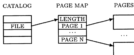
Figure 4 File system.
