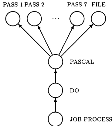
Figure 3 Compilation.
